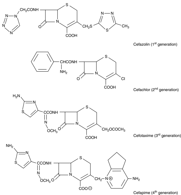
Figure 7.3 Cephalosporin structures.
